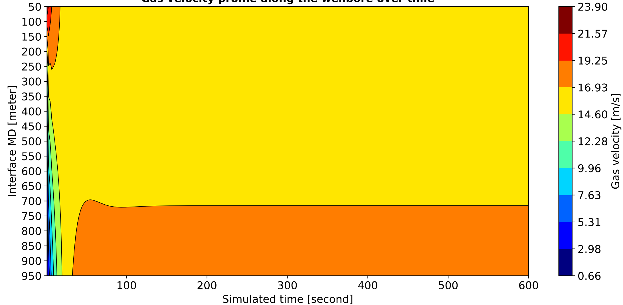
Gas velocity profile along the wellbore over time
